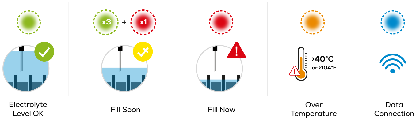
Figure 3: LED & alarm indications for flooded battery applications
