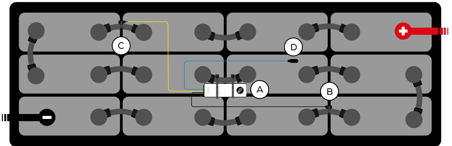
Figure 1: eGO!Core Battery Performance Monitor Final Assembly on 24V Flooded Batteries
