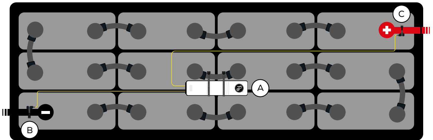
Figure 2: eGO!Plus Battery Performance Monitor Final Assembly on 24V VRLA Batteries
