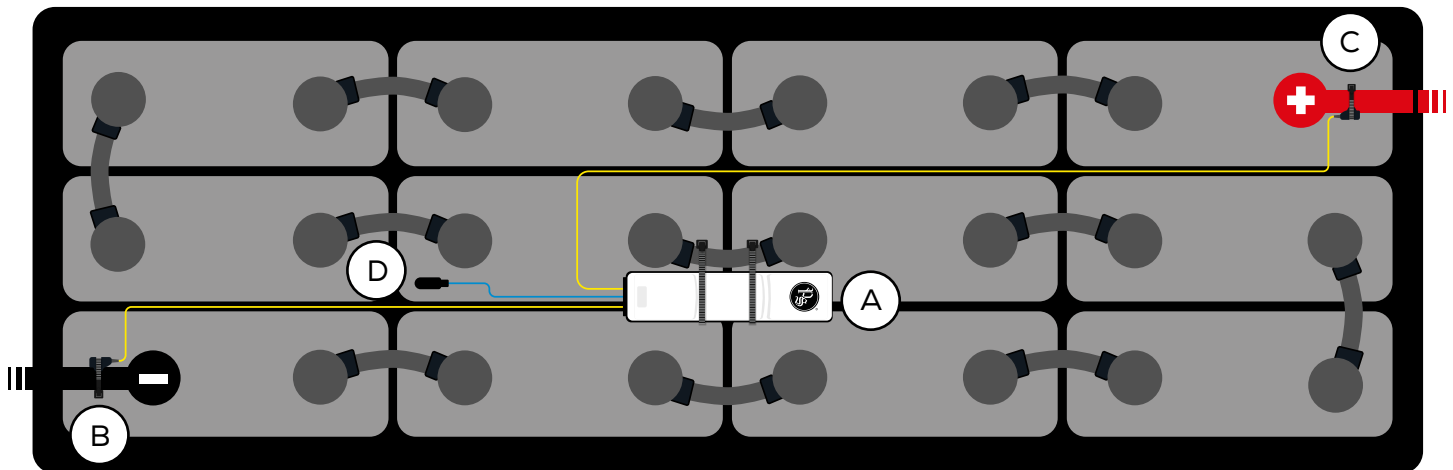
Figure 1: eGO!Plus Battery Performance Monitor Final Assembly on 24V Flooded Batteries
